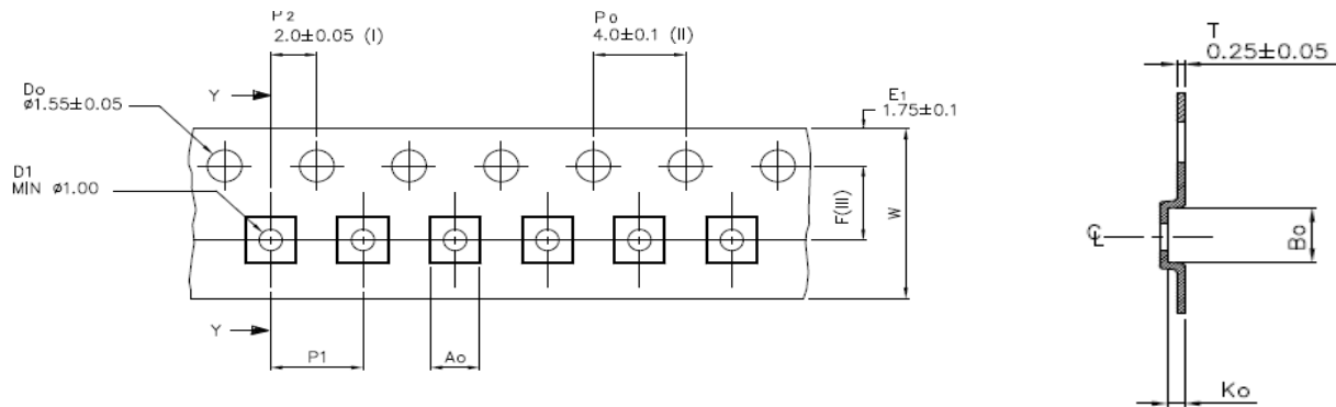
Figure 14: Tape Drawings
