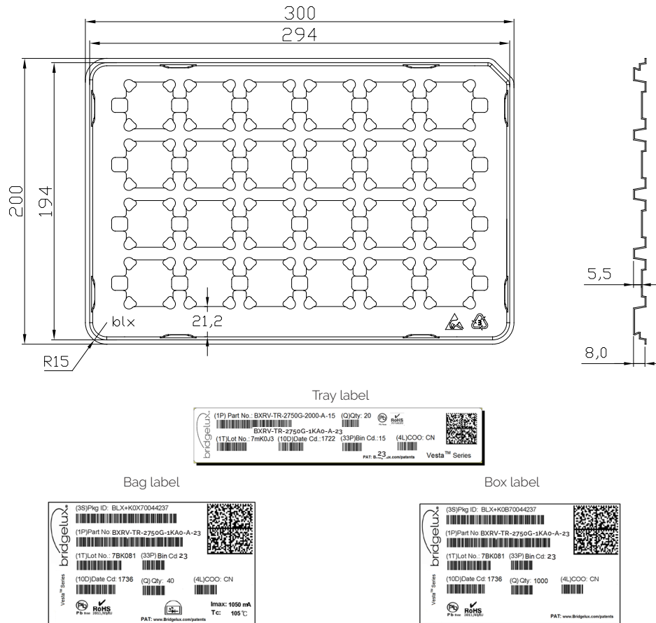
Figure 17: Vesta Series Tunable White 29mm Packaging and Labeling
