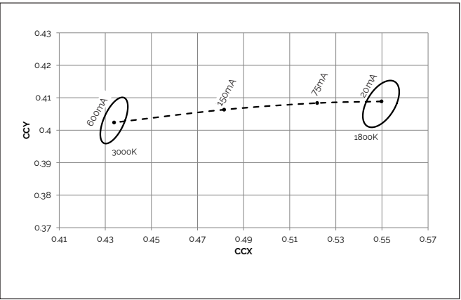
Figure 4: Color Shift vs. Forward Current 3000K - 1800K
