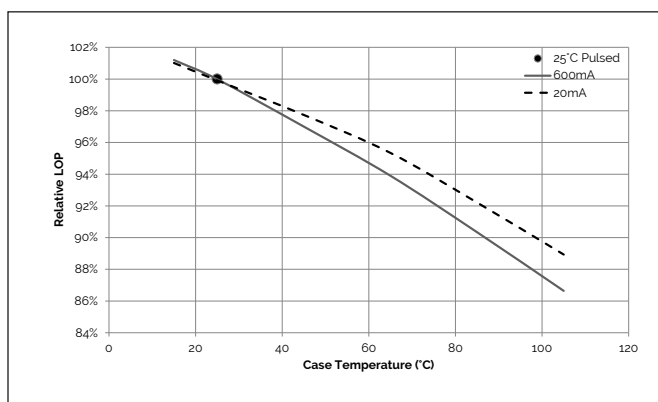
Figure 7: Relative Flux vs. Case Temperature
