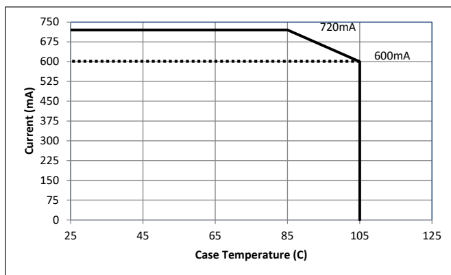
Figure 8: Derating Curve
