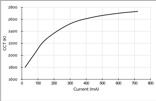
Figure 1: CCT vs. Forward Current 2700K-1800K
