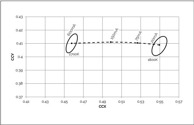
Figure 3: Color Shift vs. Forward Current 2700K - 1800K
