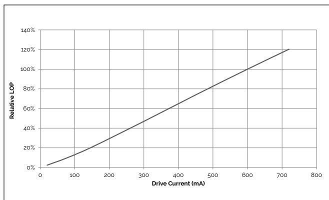
Figure 6: Relative LOP vs. Drive Current, T_c = 25^\circ\text{C}
