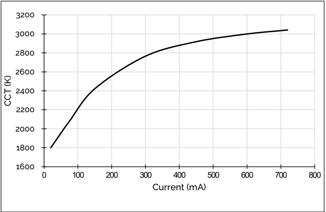
Figure 2: CCT vs. Forward Current 3000K-1800K
