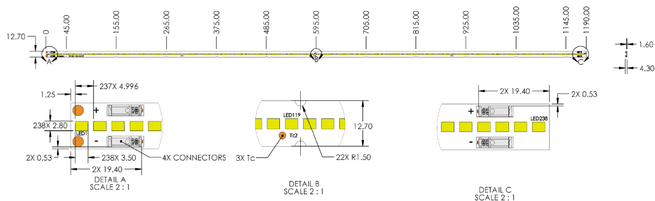
Figure 14: Drawing for BXEB-L1190U-xxx3000-C-C3
