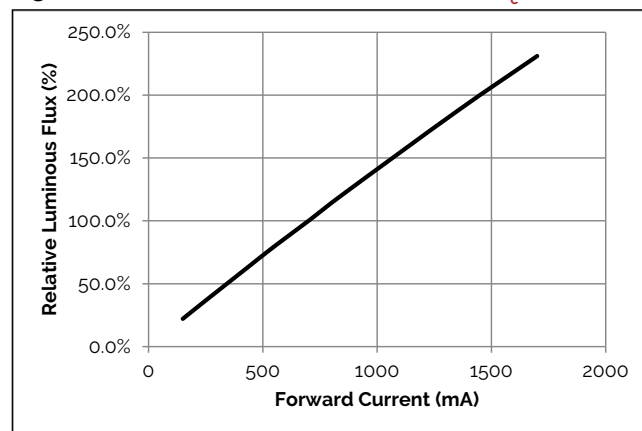
Figure 4: 590mm Relative Flux vs. Current, T_c=25^\circ\text{C}
