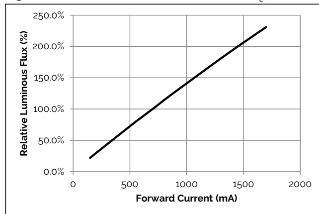
Figure 6: 1190mm Relative Flux vs. Current, T_c=25^\circ\text{C}
