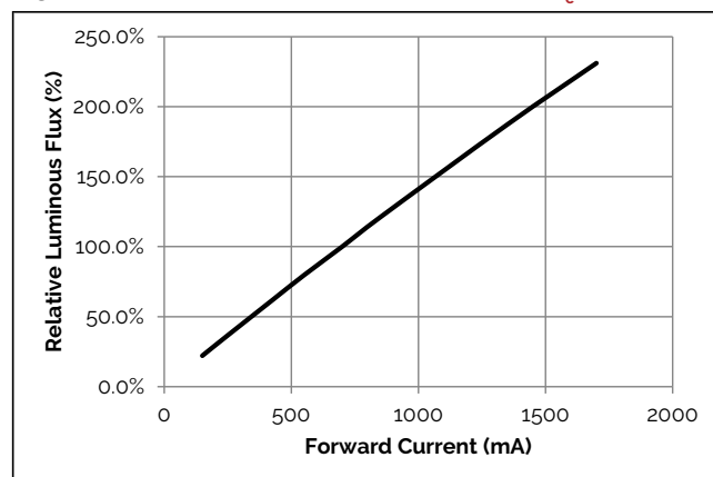
Figure 2: 340mm Relative Flux vs. Current, T_c=25^\circ\text{C}
