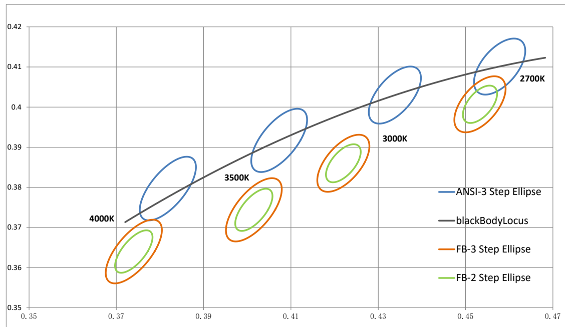
Figure 11: Warm and Neutral White Test Bins in xy Color Space
