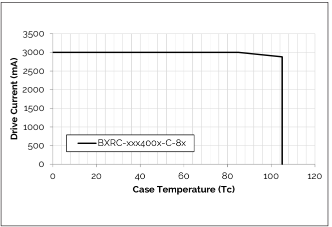
Figure 10: Derating Curve
