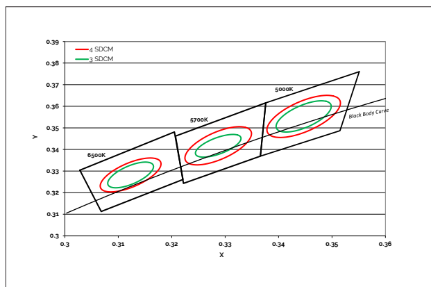
Figure 16: Cool White Test Bins in xy Color Space
