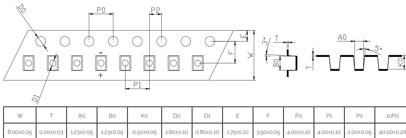
Figure 14: Tape Drawings
