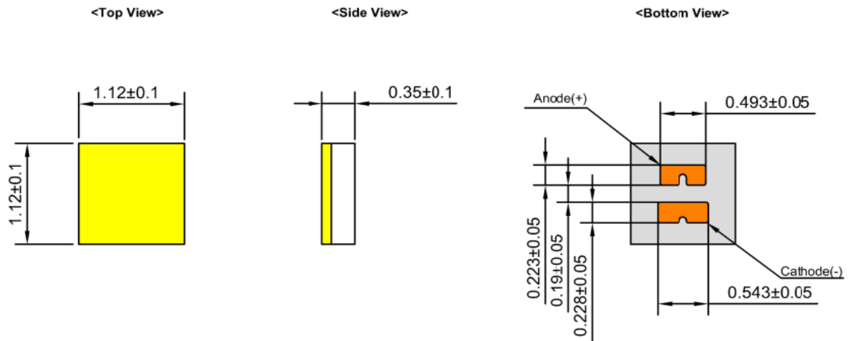
Figure 11: Drawing for CSP 1111
