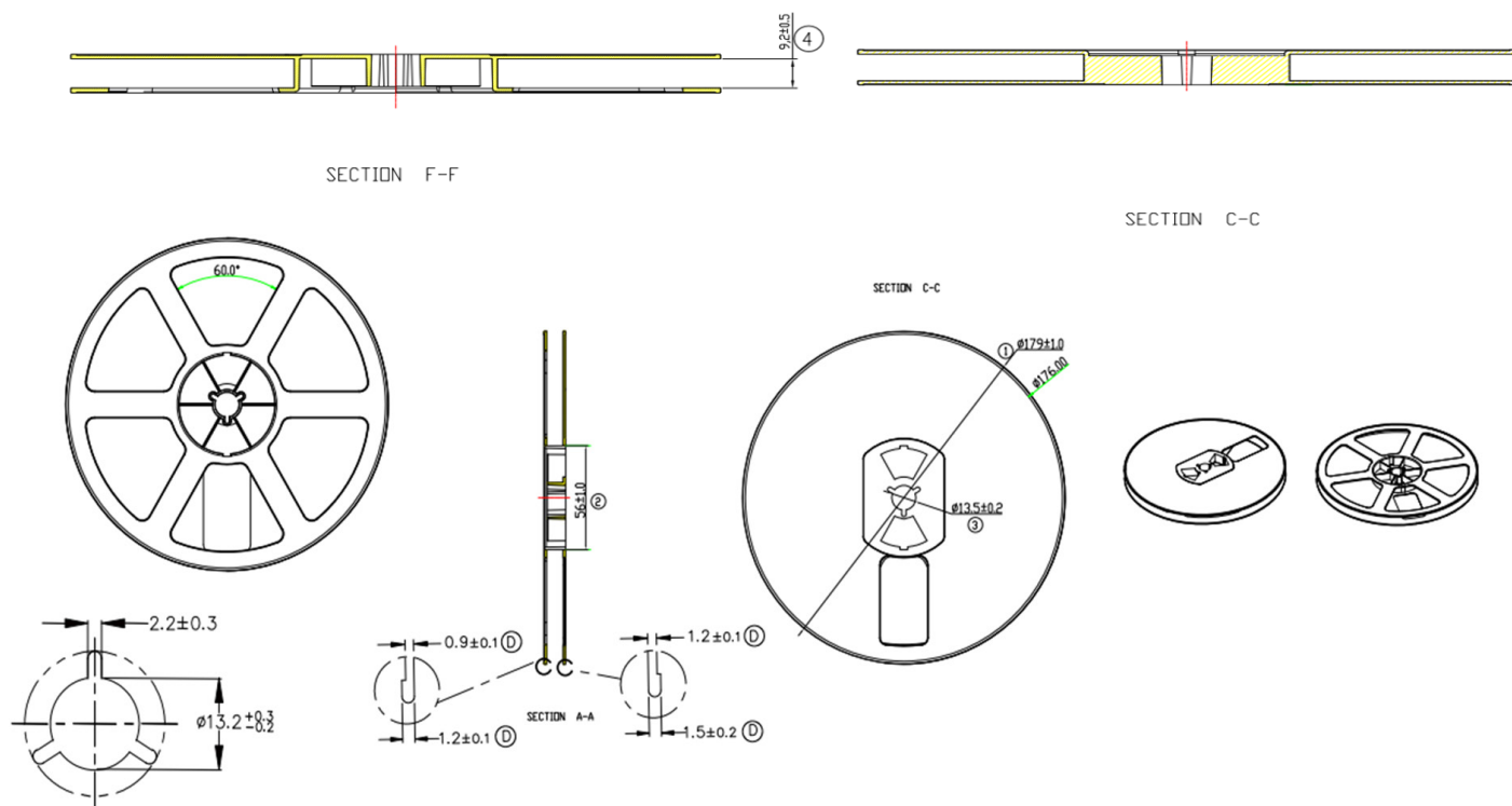
Figure 13: Reel Drawings
