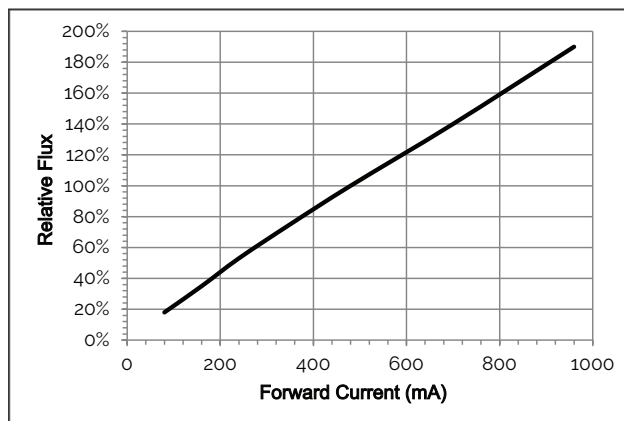
Figure 9: 280mm Relative Flux vs. Current, T_c=25^\circ\text{C}
