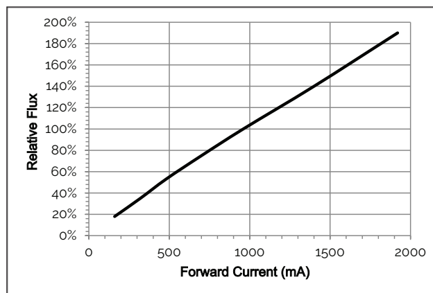
Figure 11: 560mm Relative Flux vs. Current, T_c=25^\circ\text{C}
