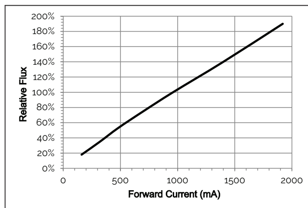
Figure 13: 1120mm Relative Flux vs. Current, T_c=25^\circ\text{C}
