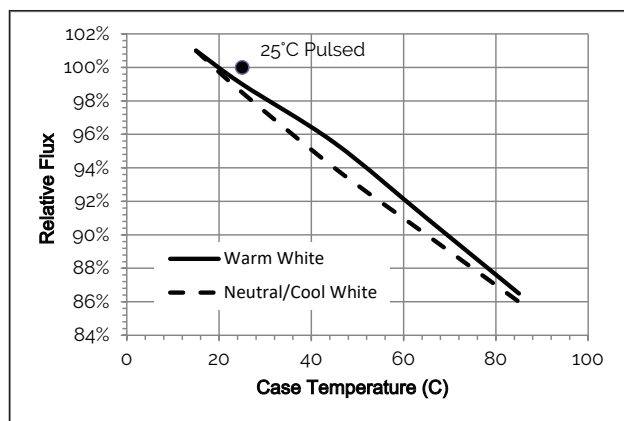
Figure 15: Relative Flux vs. Case Temperature
