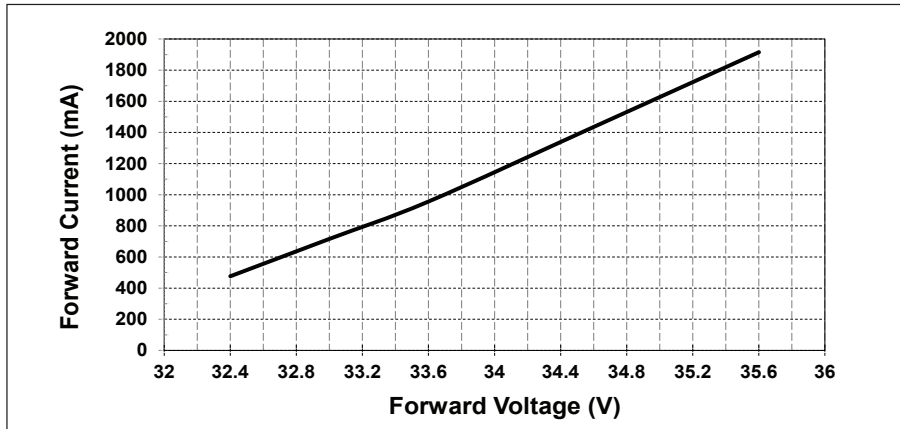
Figure 1: Current vs. Forward Voltage, T_c = 25^\circ\text{C}
