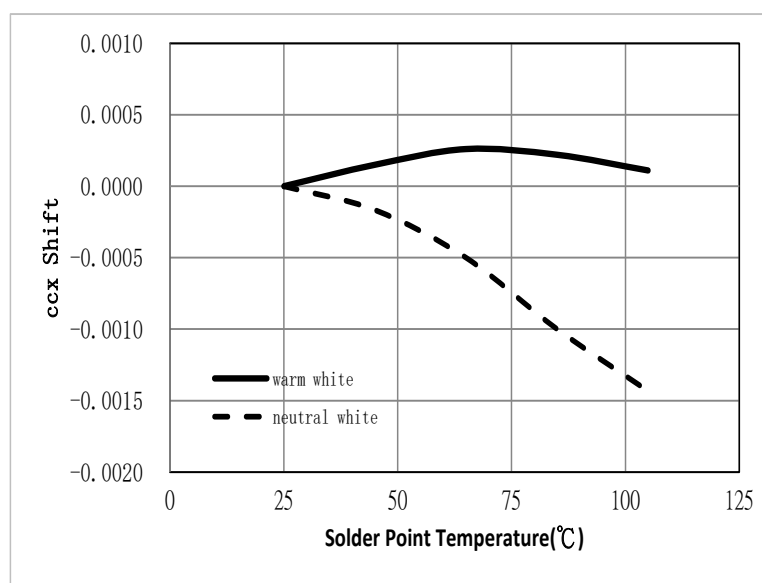
Figure 5: Typical ccx Shift vs. Solder Point Temperature
