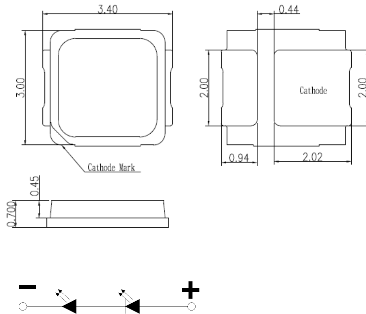
Figure 10: Drawing for SMD 3030
