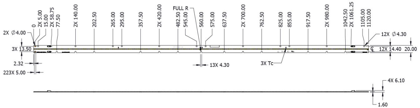
Figure 10: Drawing for EB Series Gen3 1120mm
