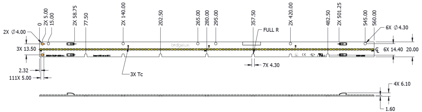
Figure 9: Drawing for EB Series Gen3 560mm
